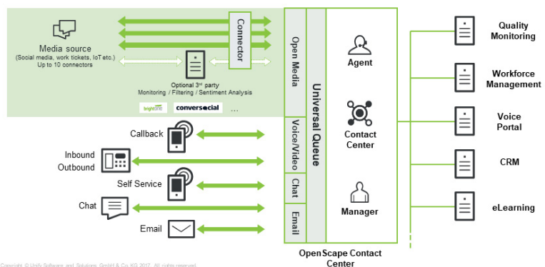
Figure 11: Open Media Framework Architecture
