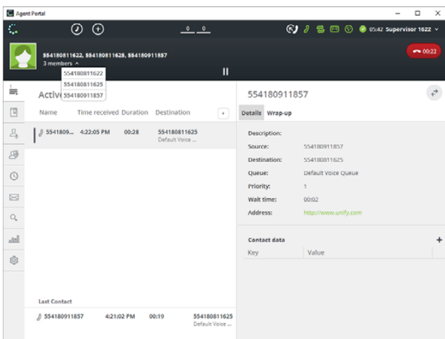
Figure 24: Agent-contact handling
